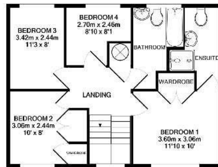
1ST FLOOR APPROX. FLOOR AREA: 65.7 SQ.M. (1600 SQ.FT.)
